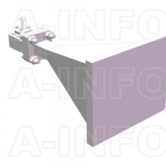
LB-34-20-C-KFSPO Standard Gain Horn Antenna 22-33GHz 20dB Gain 2.92mm Female
